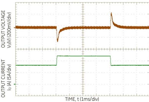
Figure 3. Dynamic Load Change Transient Response from 50% to 75% to 50% of Full Load at Room Temperature and 48 Vin; 0.1A/uS, C_{o,ext} = 470\mu\text{F} .
