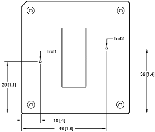
Figure 18. Case ( T_{REF} ) Temperature Measurement Location (top view).
