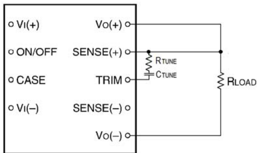
Figure 17. Circuit diagram showing connection of R_{TUNE} and C_{TUNE} to tune the control loop of the module.
